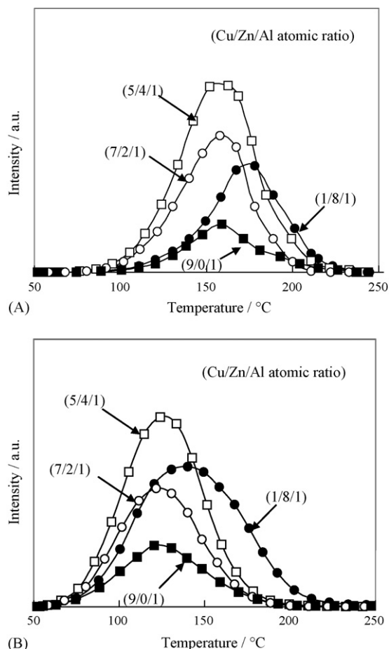
Fig. 7. TPD profiles of CH 3 OH over the hp -Cu/Zn/Al catalysts. (A) M/e = 2, H 2 ; (B) M/e = 30, HCHO.
