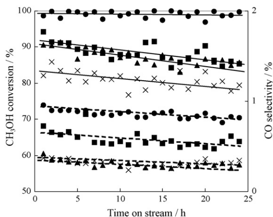
Fig. 6. Oxidative steam reforming of CH 3 OH over the Cu/Zn-based catalysts. Catalyst, 0.2 g; CH 3 OH/H 2 O/O 2 /N 2 = 10/12/5/30 ml-NTP min -1 ; reaction temperature, 200 °C. Full line, CH 3 OH conversion; dotted line, CO selectivity. (●) hp -Cu 45 /Zn 45 /Al 10 ; (■) commercial Cu/ZnO/Al 2 O 3 ; (▲) hp -Cu 50 /Zn 50 ; (×) cp -Cu 50 /Zn 50 .
