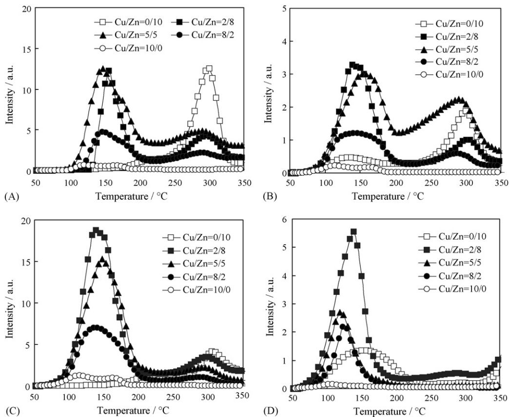
Fig. 8. TPD profiles of HCHO over the hp -Cu/Zn catalysts. (A) M/e = 2 , H_2 ; (B) M/e = 28 , CO; (C) M/e = 44 , CO_2 ; (D) M/e = 18 , H_2O .
