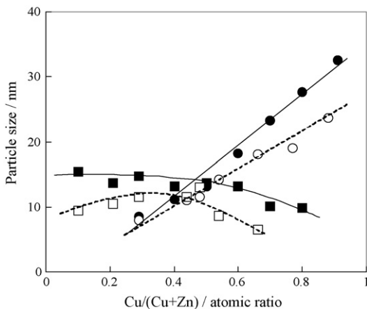
Fig. 4. Particle sizes of Cu 0 and ZnO in the hp -Cu/Zn and hp -Cu/Zn/Al catalysts after the reactions. (●) Cu 0 in hp -Cu/Zn; (○) Cu 0 in hp -Cu/Zn/Al; (■) ZnO in hp -Cu/Zn; (□) ZnO in hp -Cu/Zn/Al.
