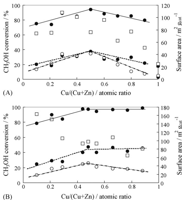
Fig. 1. CH 3 OH steam reforming over the hp -Cu/Zn (A) and hp -Cu/Zn/Al (B) catalysts. CH 3 OH/H 2 O/N 2 = 10/12/30 ml min -1 ; catalysts, 200 mg; pre-reduced with H 2 /N 2 (5/30 ml min -1 ) at 350 °C for 20 min. (●) CH 3 OH conversion (—, 250 °C; ---, 200 °C); (□) BET surface area; (○) Cu 0 surface area.
