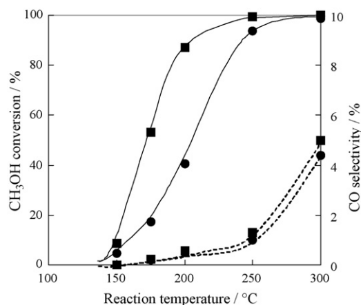
Fig. 5. Effect of the addition of O 2 in the steam reforming of CH 3 OH over the hp -Cu 50 /Zn 50 catalyst. Catalyst, 0.2 g; CH 3 OH/H 2 O/(O 2 )/N 2 = 10/12/(5)/30 ml-NTP min -1 . Full line, CH 3 OH conversion; dotted line, CO selectivity. (●) In the absence of O 2 ; (■) in the presence of O 2 .
